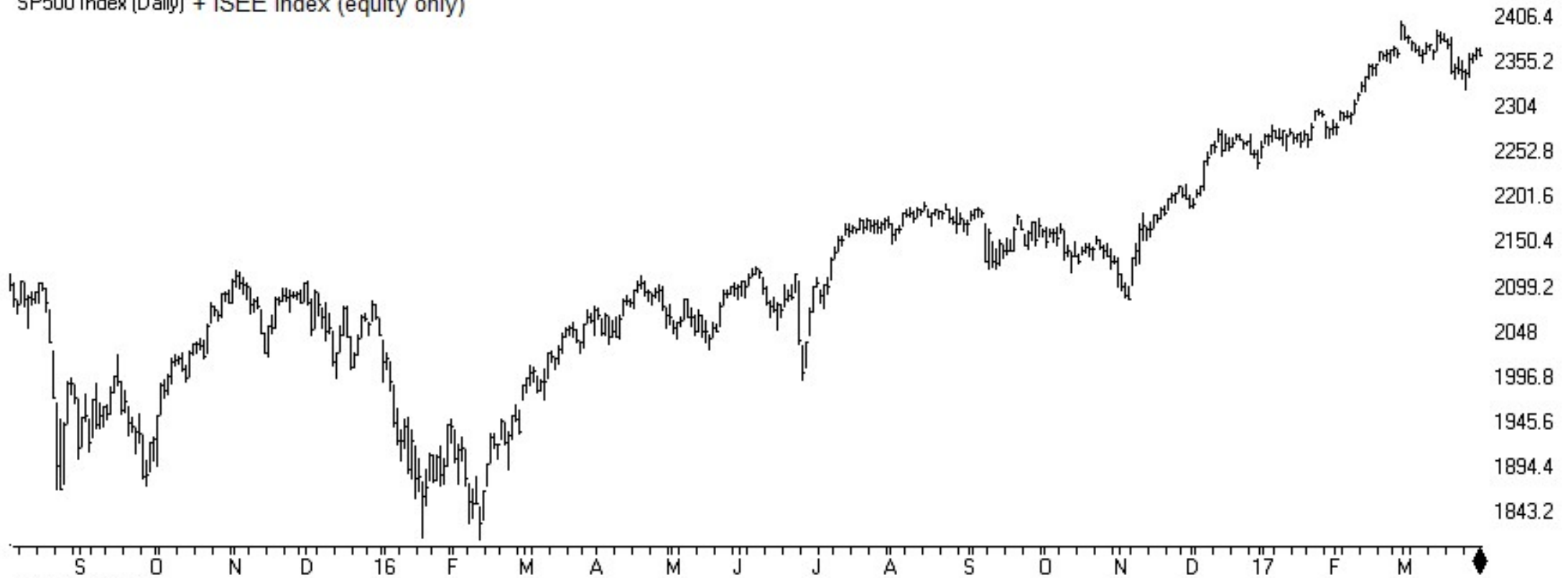
SP500 Index (Daily) + ISEE Index (equity only)
