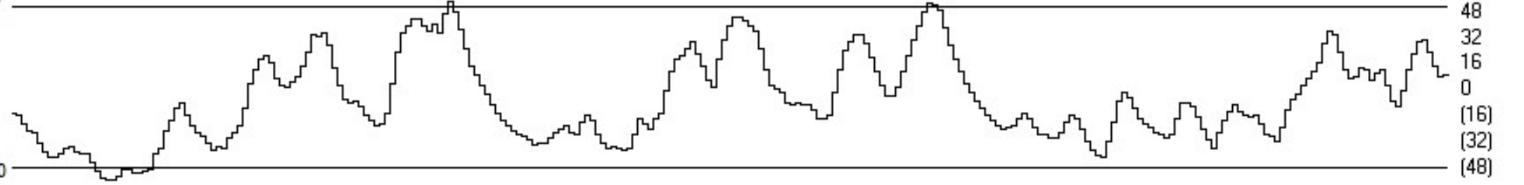
50 TCI based on VIX
