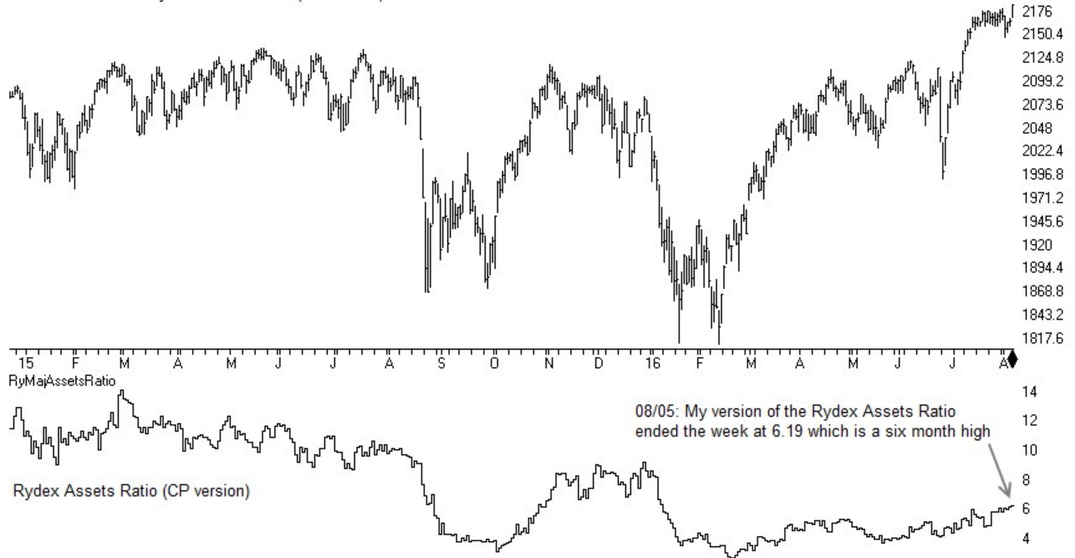
SP500 Index (Daily) + Rydex Assets Ratio (CP version)
